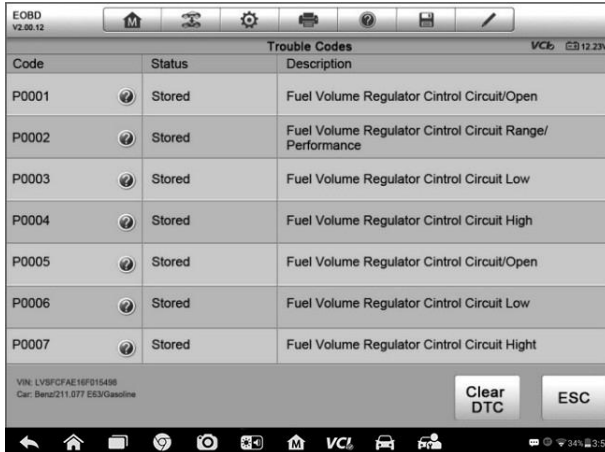
Figure 4-14 Sample DTC & FFD Screen
