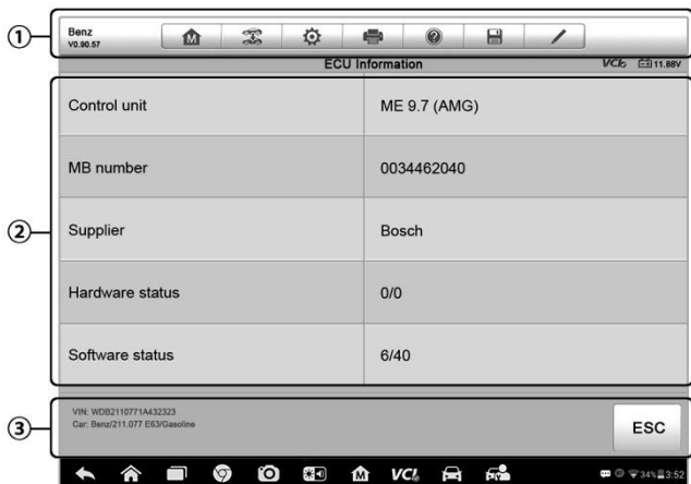
Figure 4-7 Sample ECU Information Screen
