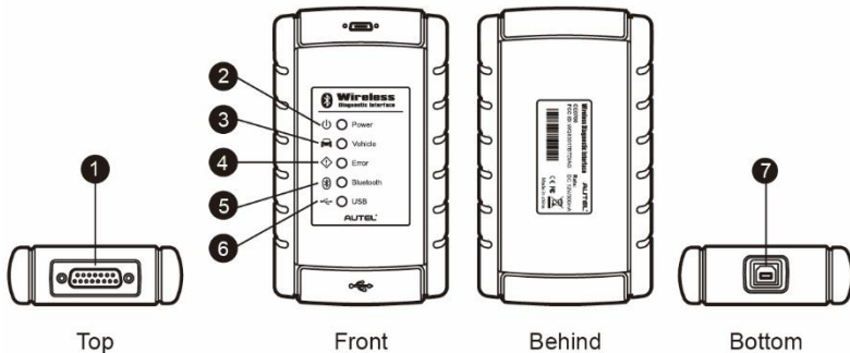
Figure 2-5 Wireless Diagnostic Interface
