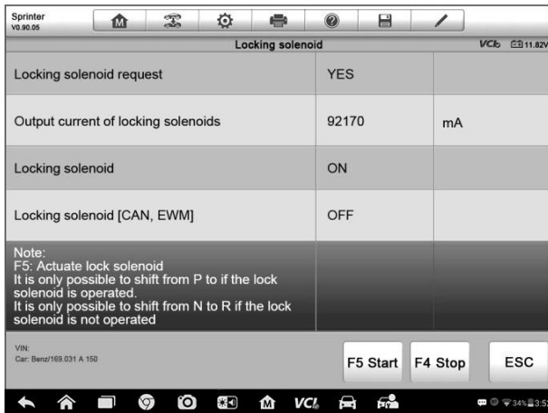
Figure 4-11 Sample Active Test Screen
